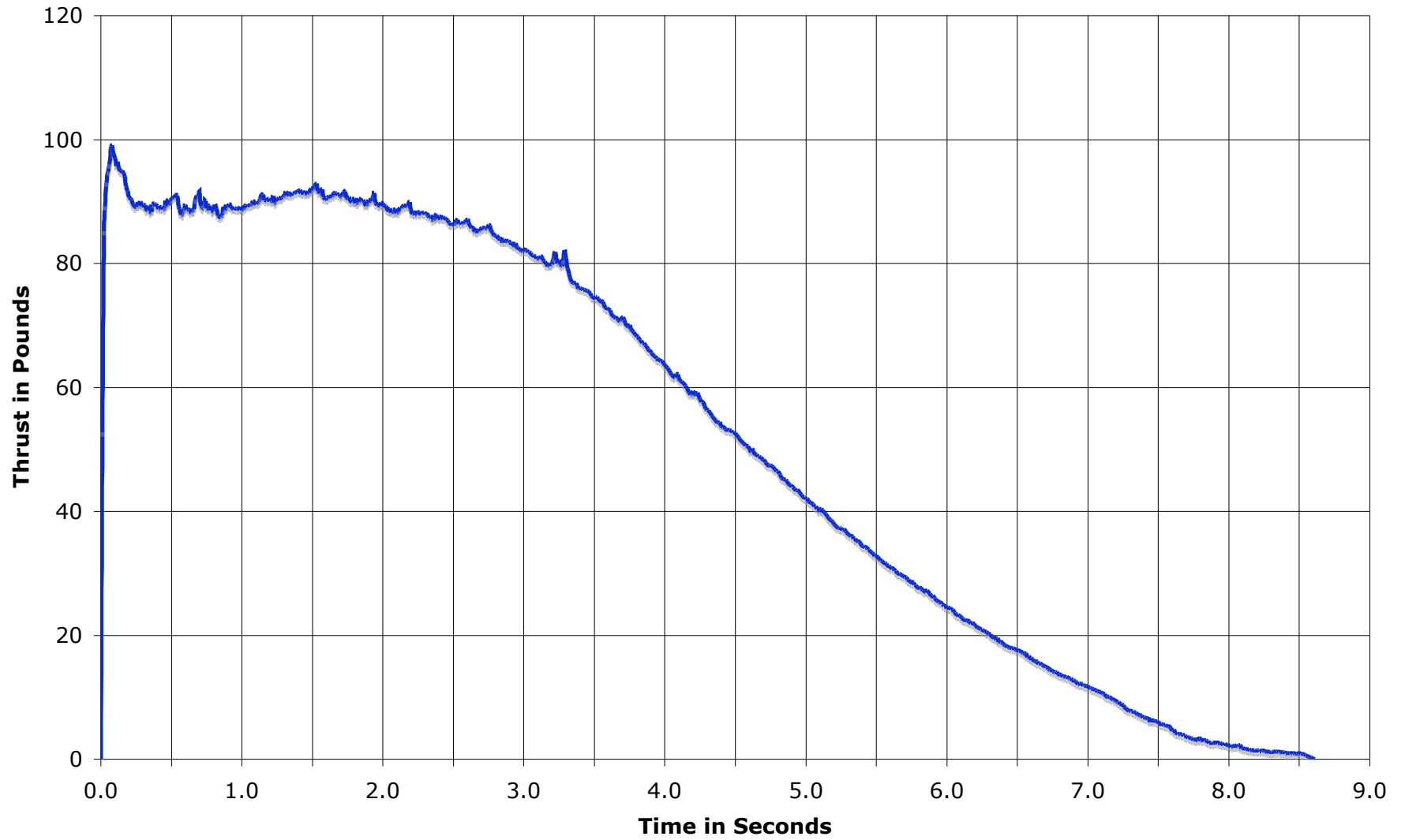
RMS-54/2560 K270W-P Time-Thrust Curve
