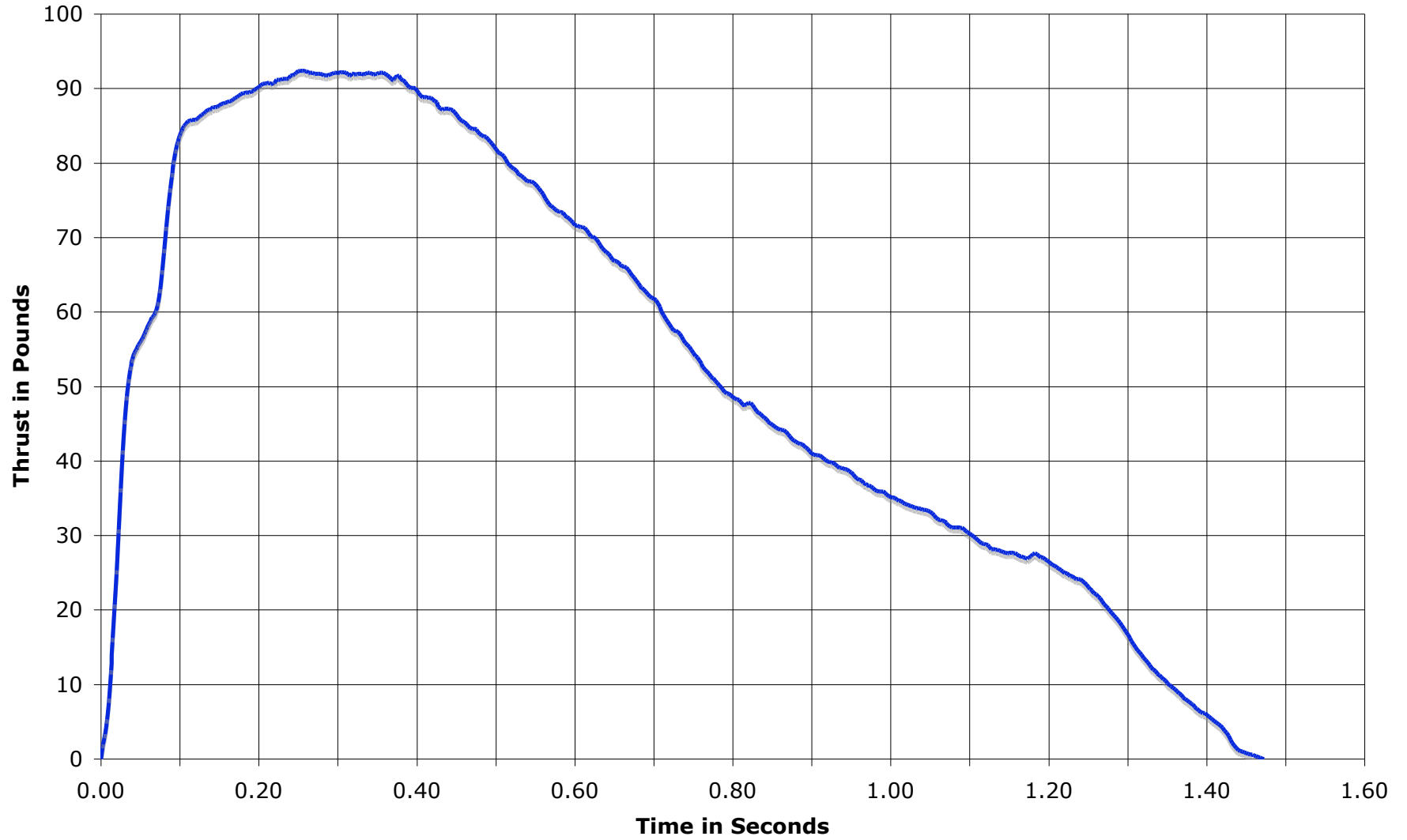
RMS-38/360 I245G-M Time-Thrust Curve
