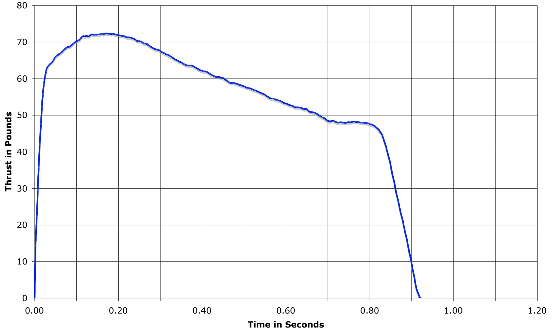
RMS-29/240 H250G-M Time-Thrust Curve
