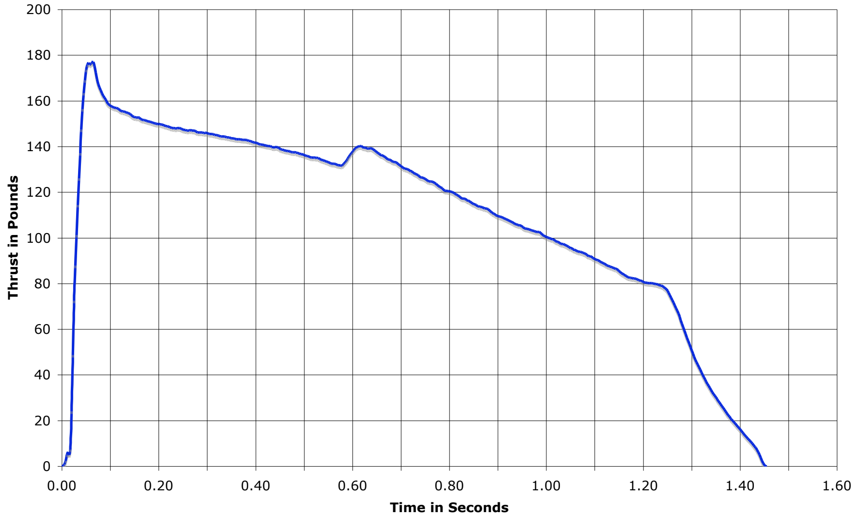
RMS-38/720 J500G-M Time-Thrust Curve
