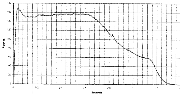
Aerotech "J420" redline
