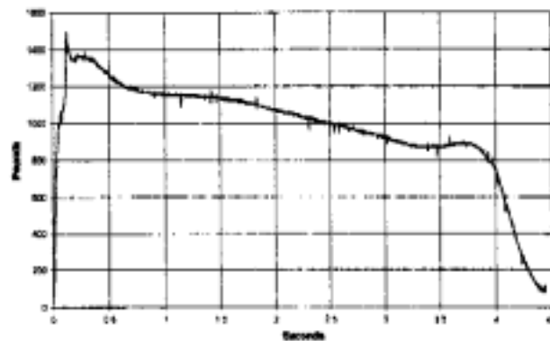
AeroTech N4800
