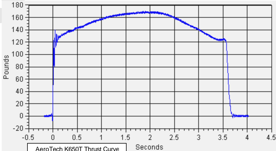
AeroTech K650T Thrust Curve Test Date: 21 Nov 98
