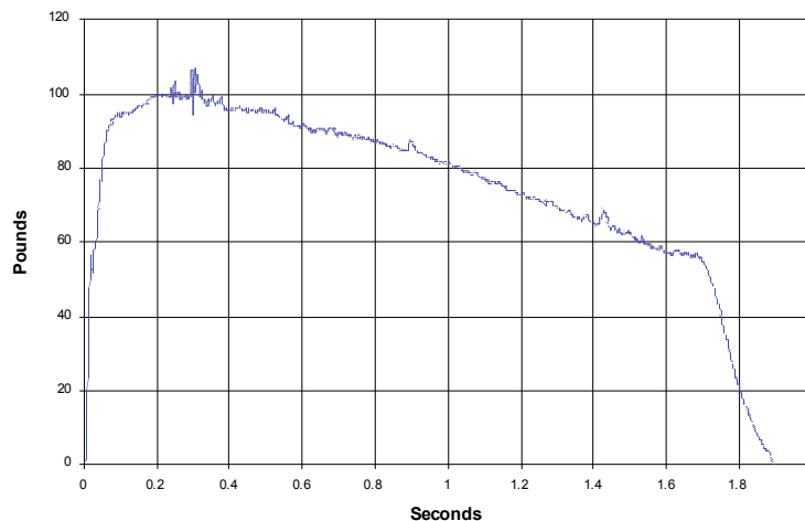
Aerotech I350R
