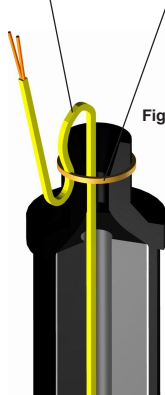
Fig.-2 FirstFire Jr. Igniter Yellow Elastic Band
